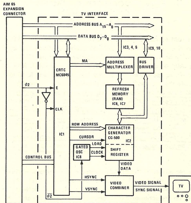
Figure 1. DISPLAY CONTROLLER INTERFACE BLOCK DIAGRAM
