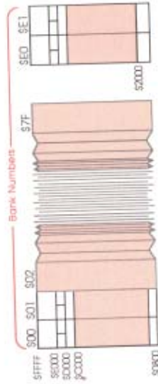
Figure 3-4 Memory allocatable through the Memory Manager
