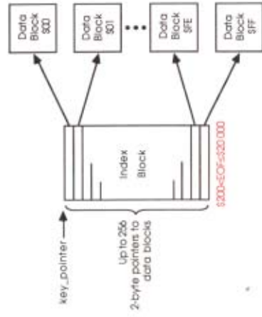
Figure A-7 Format and organization of a sapling file
