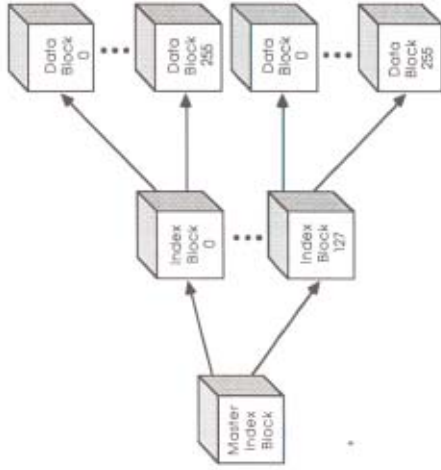
Figure 2-5 Block organization of a standard file
