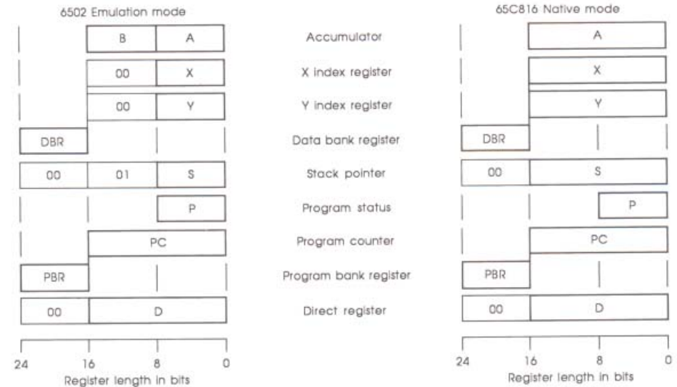
Figure 2-1 65C816 registers
