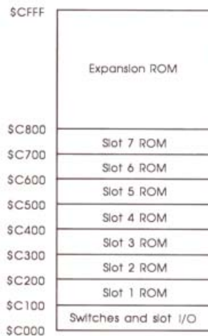
Figure 3-2 Slot ROM locations
