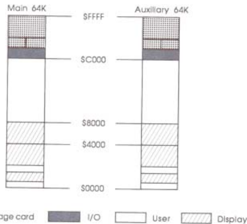
Figure 2-3 128K Apple II memory map
