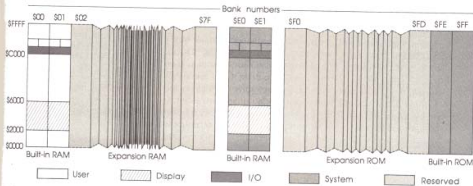
Figure 6-3 Memory map for standard Apple II programs
