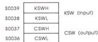
Figure 4-1 Standard I/O links
