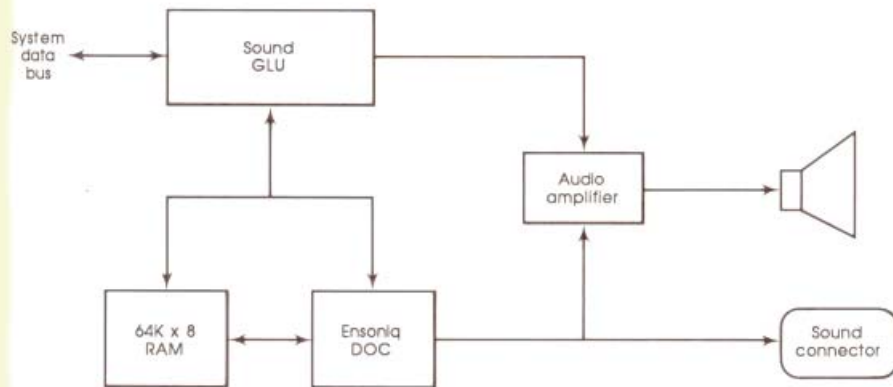
Figure 2-6 Apple IIGS sound system
