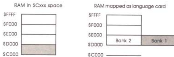
Figure 7-1 Memory map of language-card RAM
