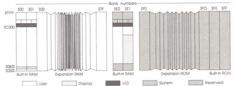
Figure 6-4 Memory map for new Apple IIGS programs
