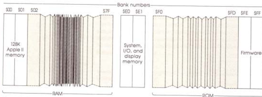
Figure 2-2 Simplified Apple IIGS memory map
