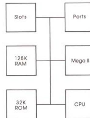
Figure 6-1 Hypothetical Apple II using the Mega II
