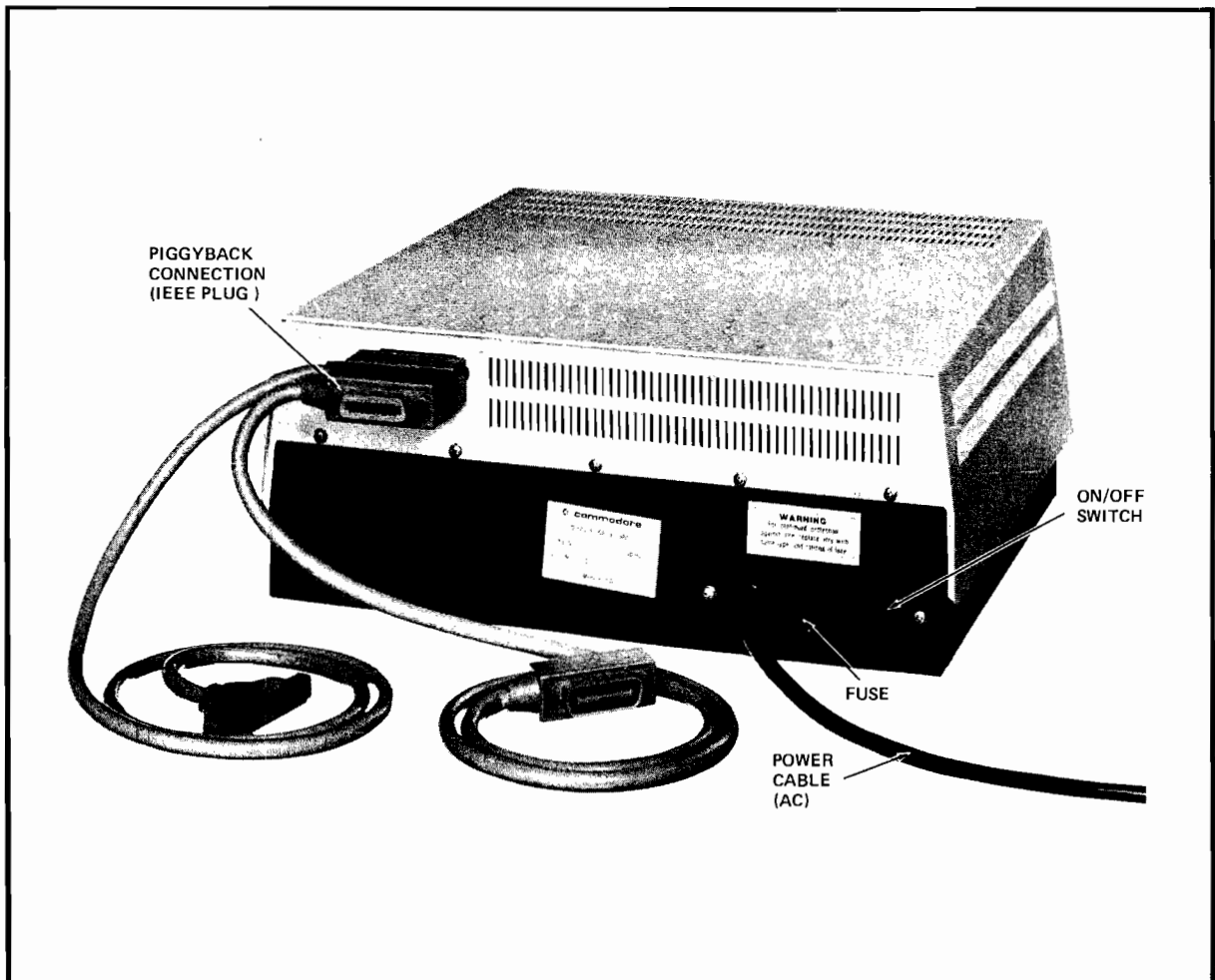
Figure 1 — Models 2040, 3040, 4040, 8050: Rear View
