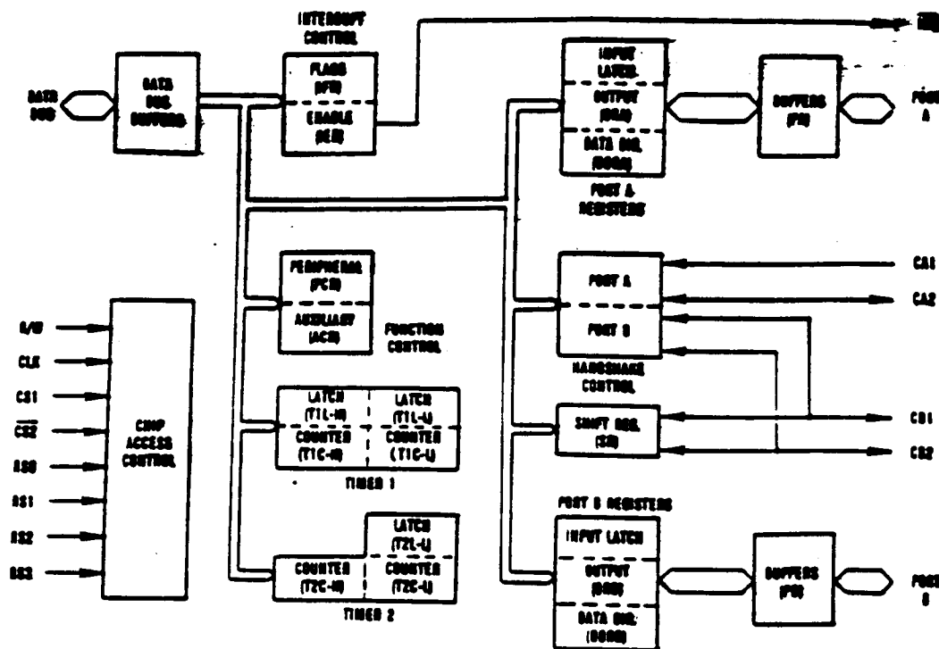
Figure 1. 6522 Block Diagram
