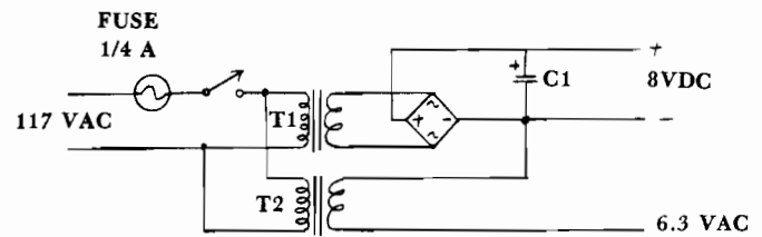
POWER SUPPLY
