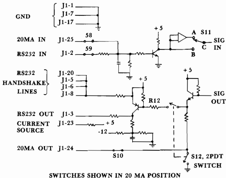
SWITCHES SHOWN IN 20 MA POSITION
