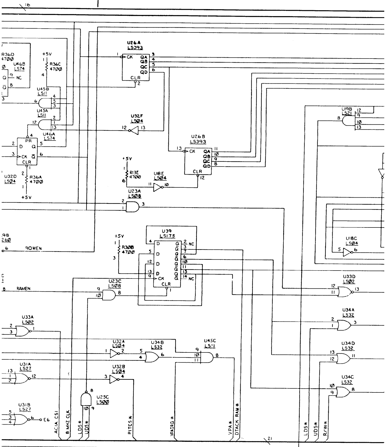
FIGURE 8-3. MEX68KECB MC68000 Educational (Sheet 2) 8-15/8-
