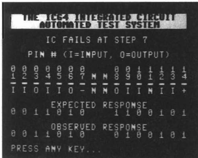
FIG. 8—THE SCREEN NOT ONLY INDICATES AN IC HAS FAILED, but it also shows what test (step) it failed and the manner in which it failed.
