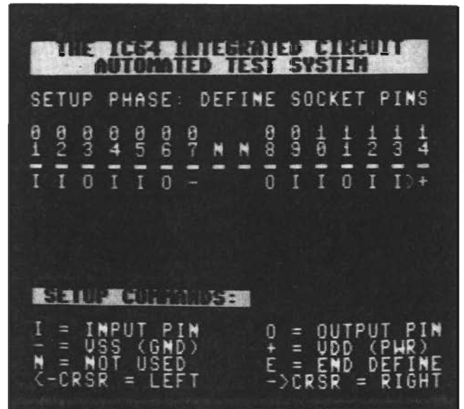
FIG. 5—FIRST STEP IN ANY TEST is to define the function of each socket pin, including the ground and +V connections.
